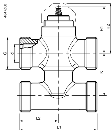
3-port valves with bypass VMP47..
