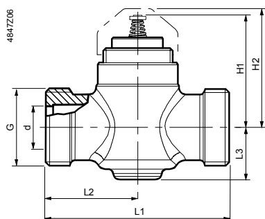
2-port valves VVP47..
