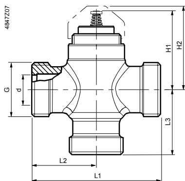
3-port valves VXP47..
